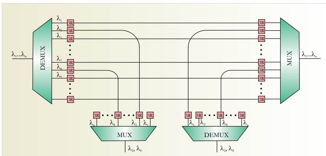
Figure 1. Example of Multi-port OADM
